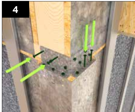
On corners, fit the clips to the beam as per the walls. Fit the 2 additional corner angle brackets WPFF001 to each side as shown using GPHS050 screws.
