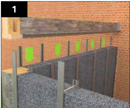
Lower the Flat Roof beam into position onto walling panels, the clips will run up both the internal and external face of the Flat Roof beam.
