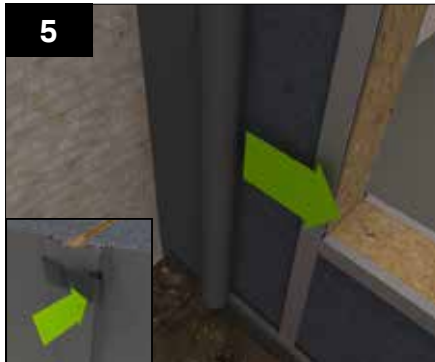
Unroll the membrane over the walls allowing this to sit slightly below DPC level (around 10 mm). Ensure that any joins in the membrane overlap by a minimum of 100mm horizontally and 150mm vertically. This can be clipped in place using the membrane clips provided. The membrane detail at the top of the wall is shown in the following steps.
