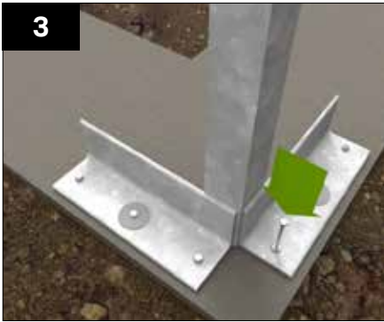
Ensure the post is positioned precisely then drill through the two smaller holes and secure in place using concrete anchors provided in SLP004 kit. Note: hup! build hidden in image for clarity.
