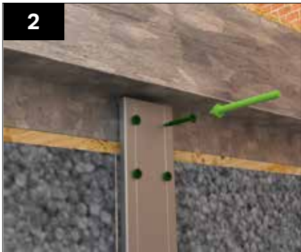
Once the beam is in position fix in place using the provided GPHS fixings into the beam with two fixings and the walling panels with two fixings for every full clip.
